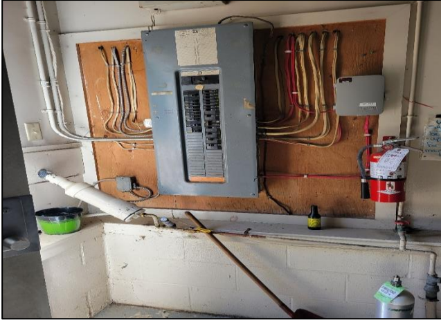
Proximity of water pipe to the electrical panel
